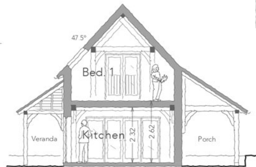
SECTION
